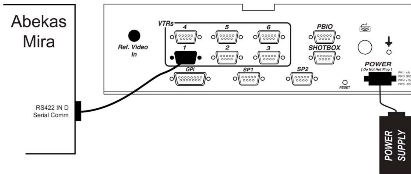
DMAT-AB Connection Diagram
