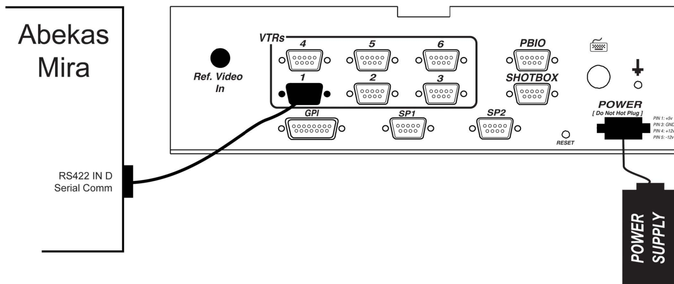
DMAT-AB Connection Diagram
